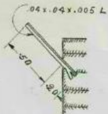
DETAIL OF STAY IN STONE WALL
